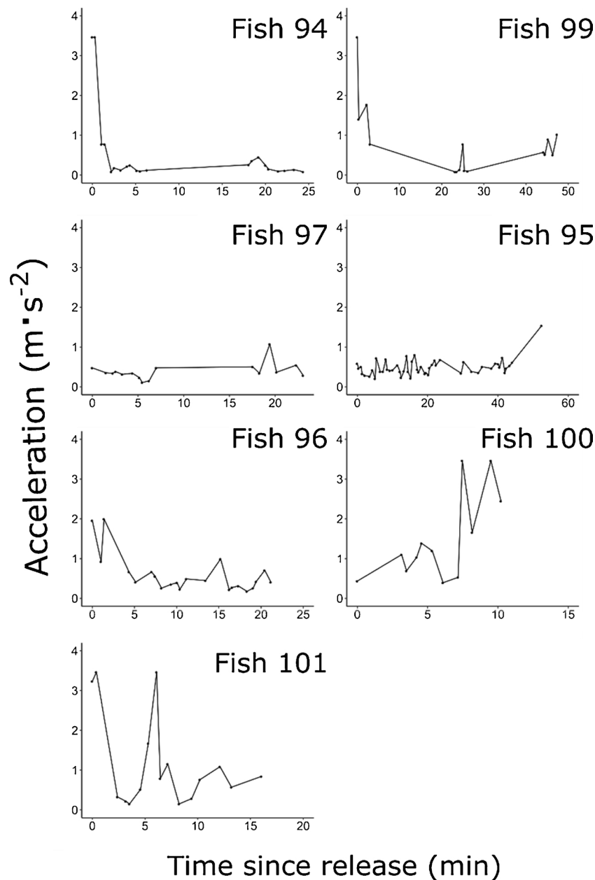
Fig. 4. Acceleration ( m\ s^{-2} ) profiles for acoustically tagged white sturgeon ( n = 7 ) manually tracked for 10–52 min after release. The points represent individual acoustic detections and are connected by lines for visualization. Plots are ordered based on sturgeon size, from smallest (156 cm FL – Fish 94) to largest (257 cm FL – Fish 101).
